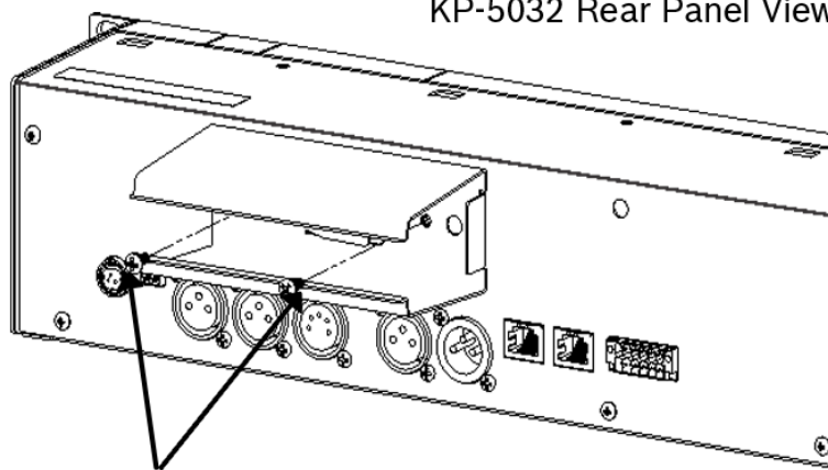
Mounting Screws
